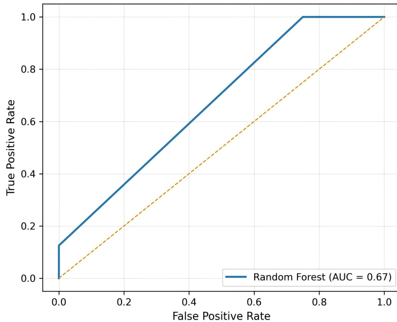
Figure 5. Receiver operating characteristic (ROC) curve for the Random Forest approach.
