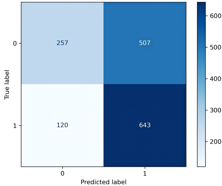
Figure 4. Confusion matrix for the Random Forest approach.
